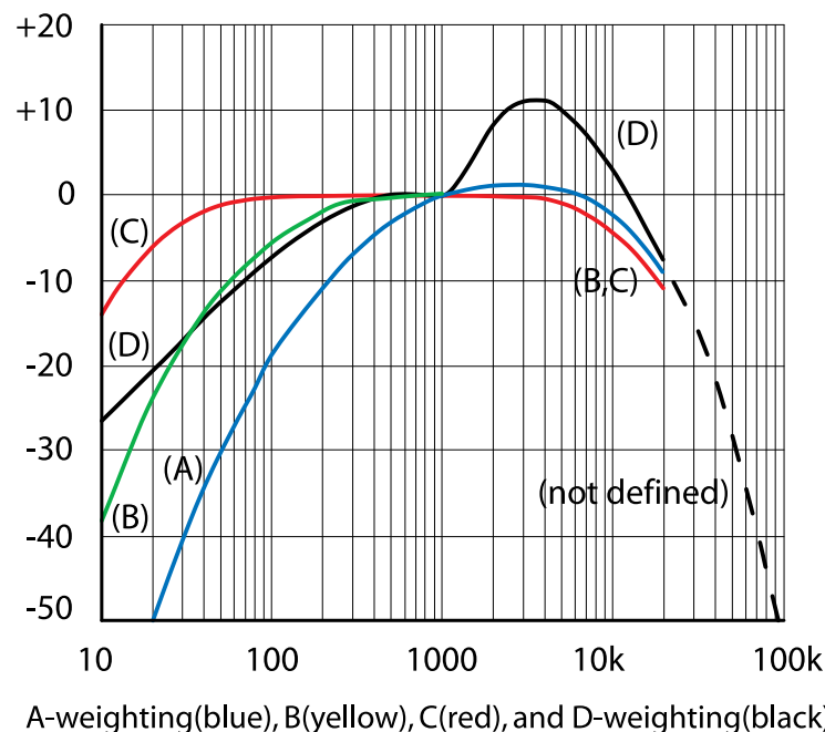
A-weighting curve
