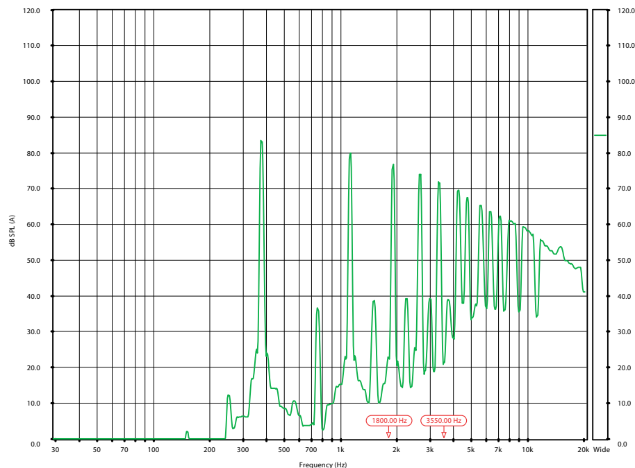
Figure 2: Fourier analyse square wave 374 Hz
