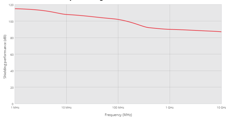
■ 7600 series - U-shape EMI gasket
